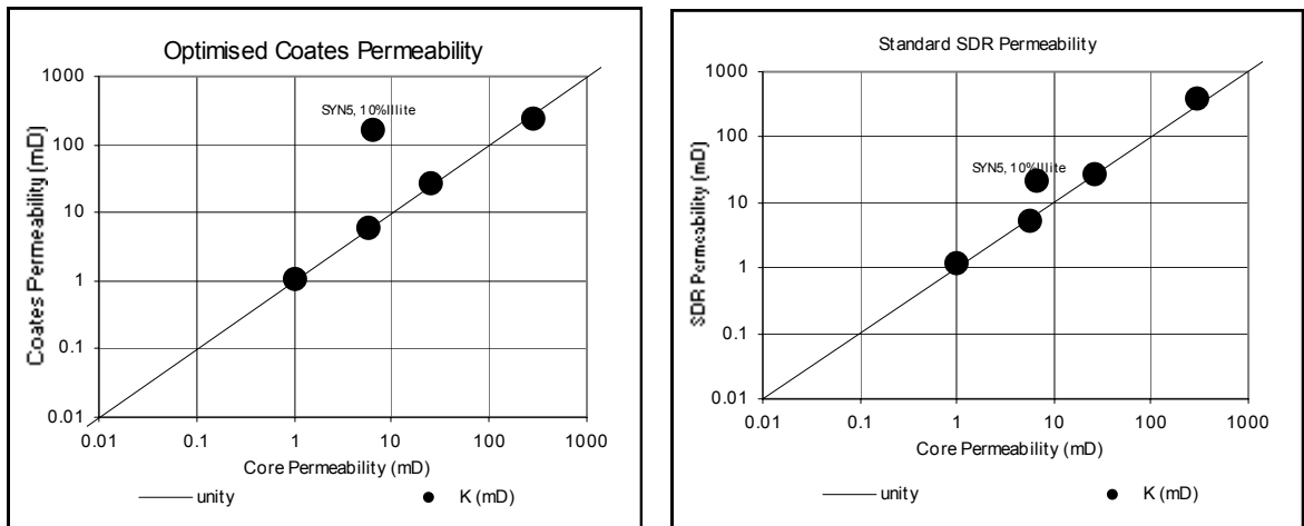
Figure 2: Modelled NMR Permeability Against Core Permeability.
