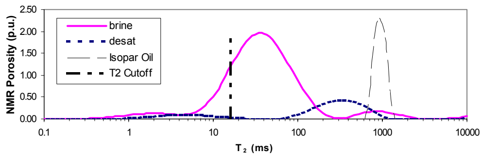
Figure 1e: T2 Distribution for Syn 5, 10% Illite.
